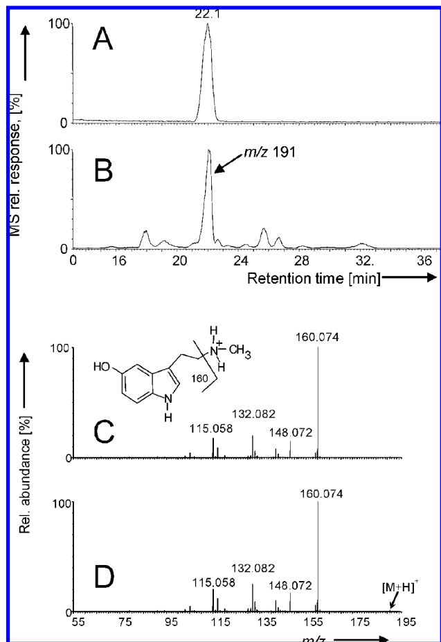
Figure 4. Positive ion electrospray LC-MS analysis and tandem mass spectra of fraction 7 and N ω -methylserotonin: total ion chromatograms of (A) N ω -methylserotonin standard and (B) fraction 7. A comparison of the product ion tandem mass spectra of N ω -methylserotonin and a compound from fraction 7 eluting at 22 min is shown; the major fragment ion corresponds to the loss of methylamine from the side chain: (C) N ω -methylserotonin standard; (D) black cohosh fraction 7.
