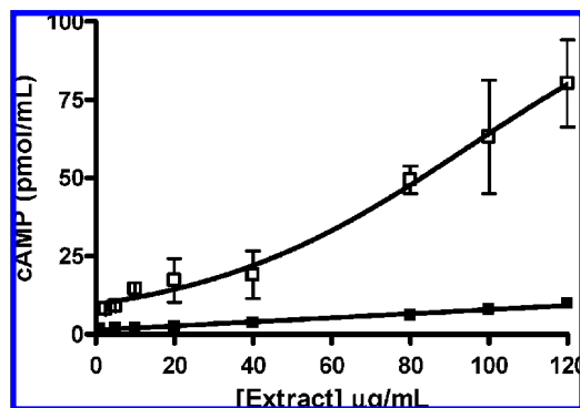
Figure 3. Black cohosh induces intracellular cAMP: dose-dependent induction of cyclic AMP (pmol/mL) for the clinical black cohosh extract (■) and XAD-MeOH extract, EC_{50} = 70 \mu\text{g/mL} (□) mediated through the 5-HT 7 receptor.
