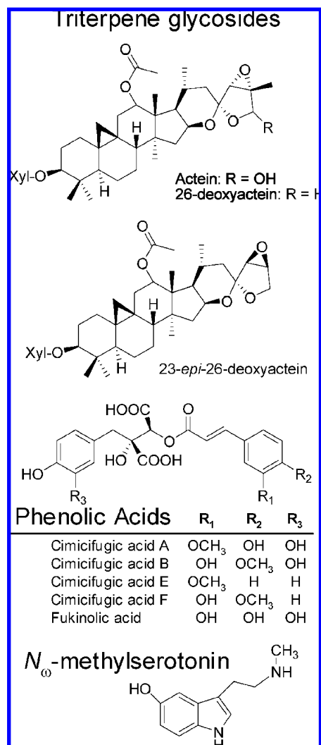
Figure 1. Key phytoconstituents of black cohosh.
