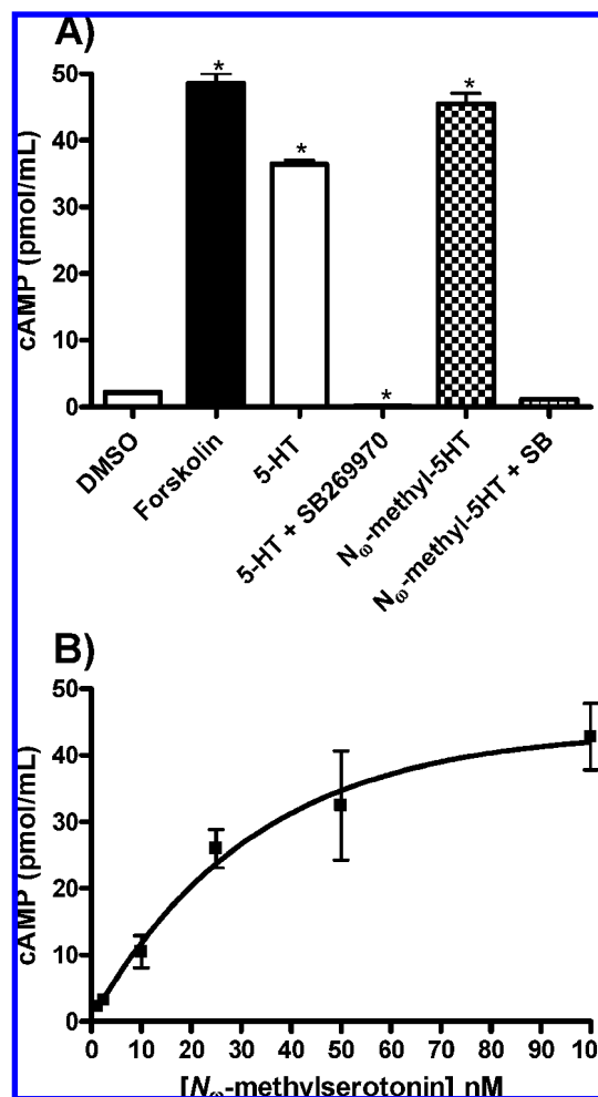
Figure 6. N ω -Methylserotonin induces intracellular cAMP: (A) cyclic AMP intracellular levels of human 5-HT 7 transfected HEK293 cells after treatment with DMSO, forskolin (20 nM), 5-HT (10 nM), N ω -methylserotonin (100 nM); and cotreatment with 5-HT 7 receptor antagonist, SB 269970 (5 μM); (B) intracellular cyclic AMP (pmol/mL) as a response of increasing dosage from N ω -methylserotonin mediated through the 5-HT 7 receptor. *, p < 0.05.
