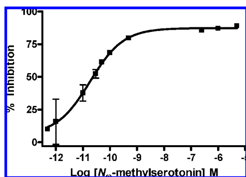
Figure 5. N ω -Methylserotonin can bind to the 5-HT 7 receptor: percent inhibition of 5-HT 7 receptor binding with increasing doses of N ω -methylserotonin. IC 50 = 23 pM.
