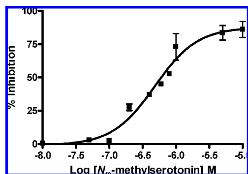
Figure 7. N_{\omega} -Methylserotonin exhibits SSRI activity: dose-dependent percent inhibition of selective serotonin re-uptake with N_{\omega} -methylserotonin. The IC_{50} value was determined to be 490 nM.
